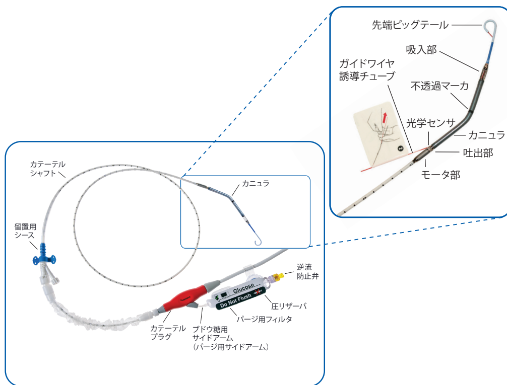
図2.3 IMPELLA CP SmartAssist
